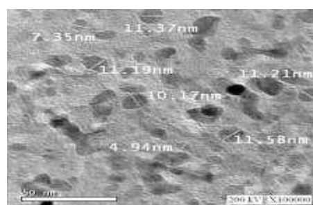
Fig. 1: Determination of size and shape of Mn NPs suspension using Transmission electron microscope (TEM)
