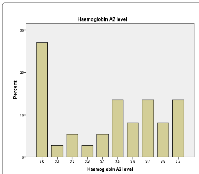
Figure 2: Frequency of \beta -mutation at different HbA2 level (n=37).
