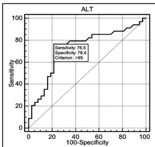
Fig. 1: ROC Analysis.
