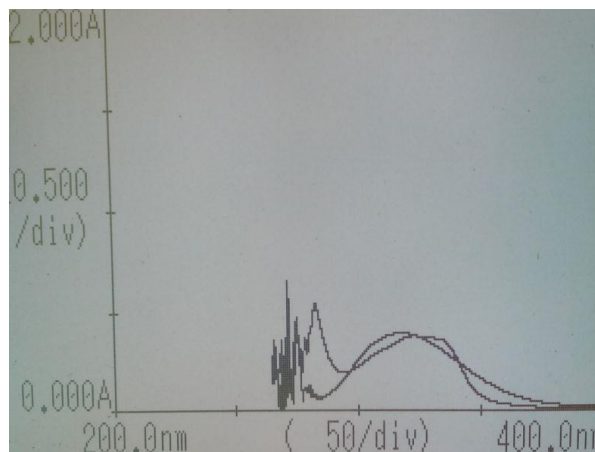
Fig. 1: Overlain spectra of norfloxacin and tinidazole with 10% phenol and 20% sodium benzoate blend.
