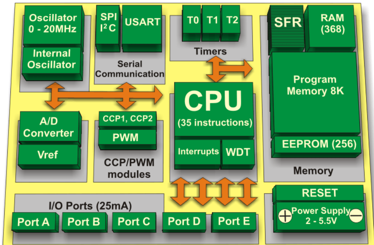
Fig. 6(3): PIC16F887 Block Diagram
